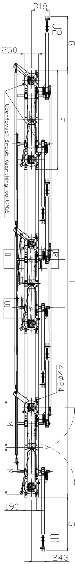
Three pole disconnector in line 3SHT(U)-XXXX.K
